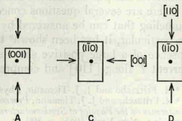
FIG. 1. Definitions of the uniaxial stress coefficients \Delta I/IX . The arrows represent uniaxial compressional stress of unit magnitude.
